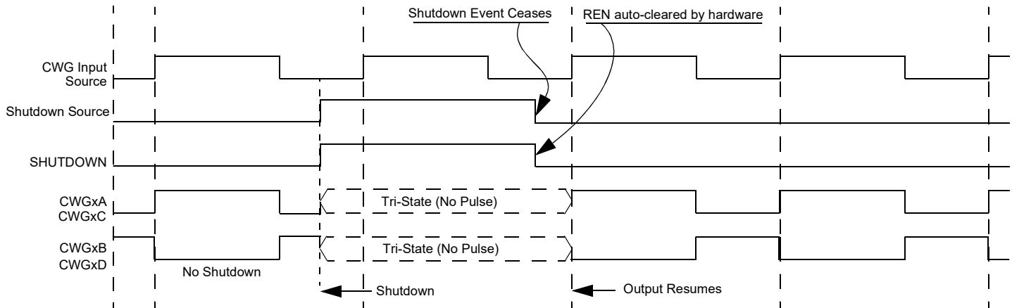
FIGURE 26-16: SHUTDOWN FUNCTIONALITY, AUTO-RESTART ENABLED (REN = 1, LSAC = 01, LSBD = 01)
