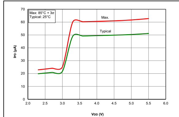
FIGURE 45-52: I po Base, NP Sleep Mode, PIC18F26/27/45/46/47/55/56/57K42 Only.
